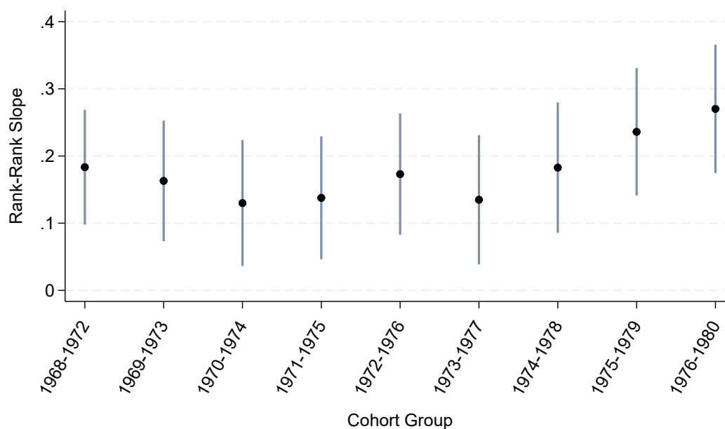
Figure A5: Rank-rank slope estimates for child age range 30-40
