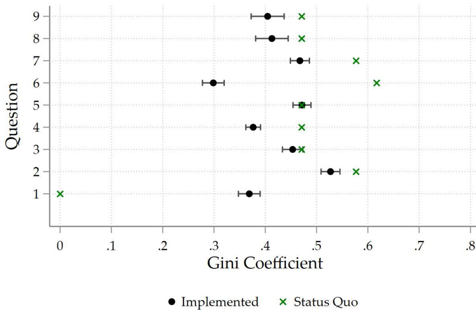
Figure 6: Gini Coefficient
